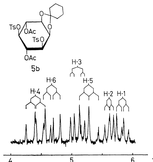
Fig. 3. Partial PMR spectrum of 4,6-di- O -acetyl-1,2- O -cyclohexylidene-3,5-di- O - p -toluenesulfonyl- myo -inositol ( 5b ) (60 MHz, \text{CDCl}_3 ).
