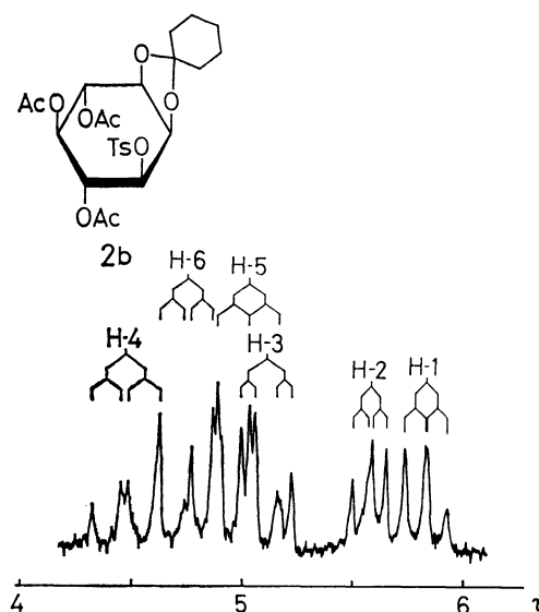
Fig. 2. Partial PMR spectrum of 4,5,6-tri- O -acetyl-1,2- O -cyclohexylidene-3- O - p -toluenesulfonyl- myo -inositol ( 2b ) (60 MHz, \text{CDCl}_3 ).
