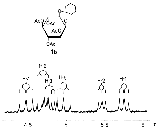
Fig. 1. Partial PMR spectrum of 3,4,5,6-tetra- O -acetyl-1,2- O -cyclohexylidene- myo -inositol ( 1b ) (100 MHz, \text{CDCl}_3 ).
